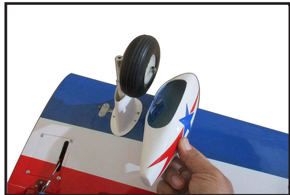
3) Attach Fiberglass Wheel Pants into landing Gear.
