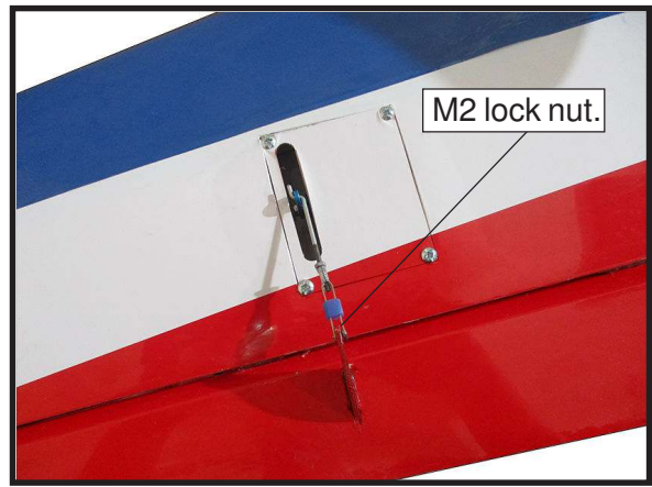
FLAP PUSHROD HORN INSTALLATION.
